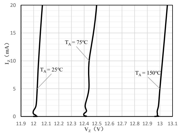
Fig 2 Typical Zener Breakdown
