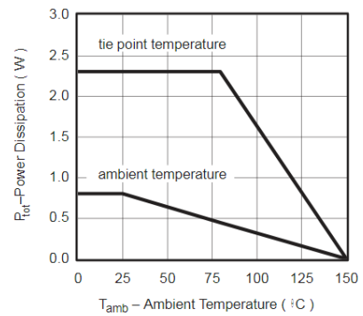
Figure 4. Power Dissipation vs. Ambient Temperature
