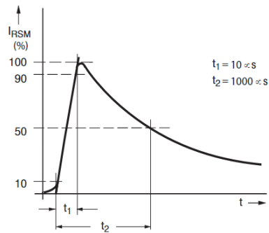
Figure 3. Non-Repetitive Peak Reverse Current Pulse Definition
