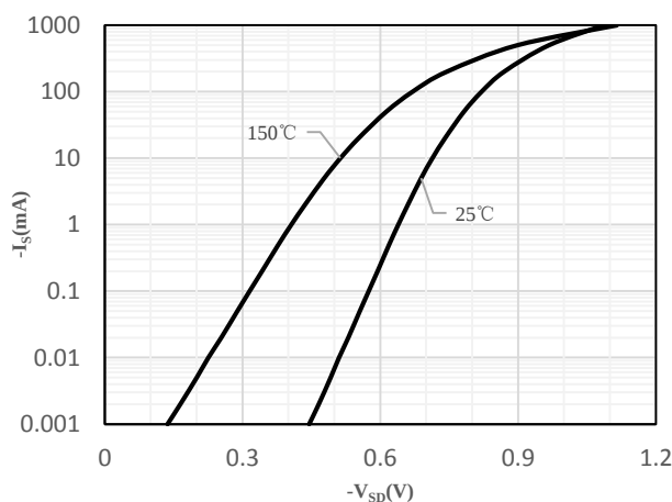
Fig 4 Body-Diode Characteristics
