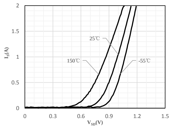
Fig 6 Body-Diode Characteristics
