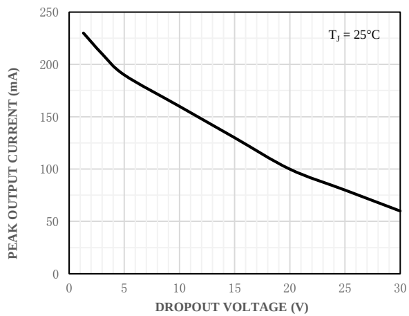
Fig 11 Peak Output Current vs. Dropout Voltage
