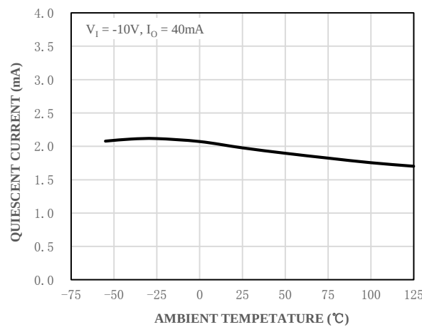
Fig 5 Quiescent Current vs. Temperature
