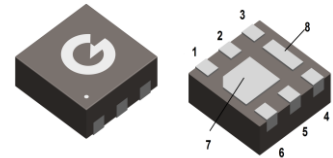
DFN2020-6L
