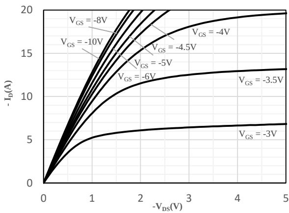
Fig 3 Output Characteristics
