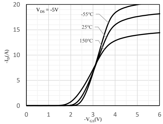
Fig 8 Transfer Characteristics
