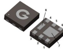
DFN2020-6L
