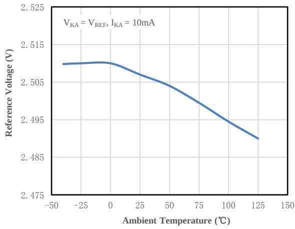
Fig 1 Reference Voltage vs. Temperature
