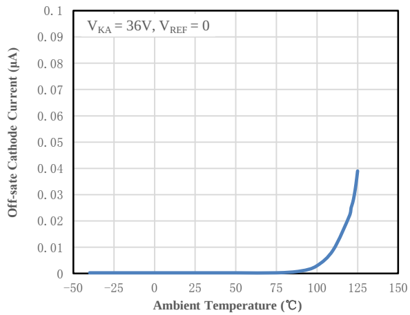
Fig 3 Off-state Cathode Current vs. Temperature
