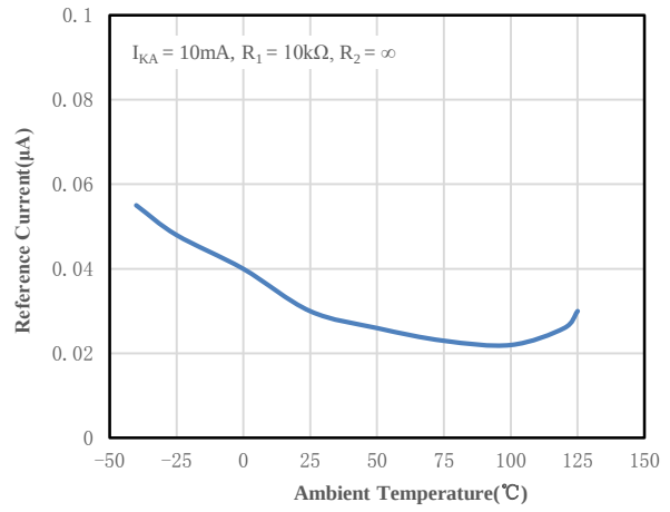
Fig 2 Reference Current vs. Temperature
