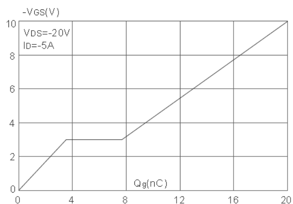
Fig 8 Gate-Charge Characteristics
