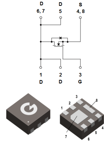
DFN2020-6L
