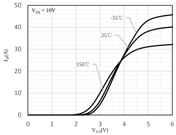
Fig 8 Transfer Characteristics
