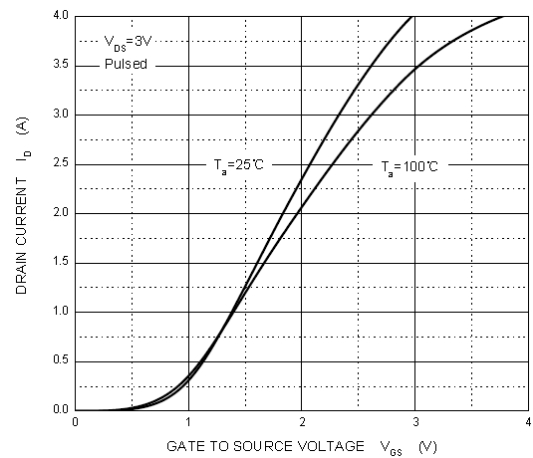
Fig 6 Transfer Characteristics
