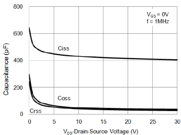
Fig 7 Capacitance Characteristics
