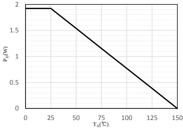
Fig 1 Power Dissipation
