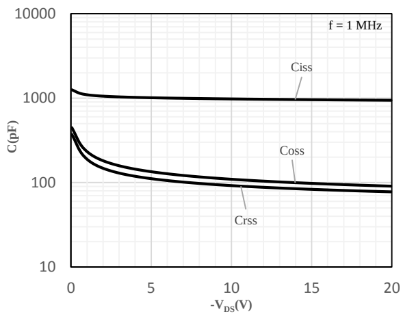
Fig 9 Capacitance Characteristics
