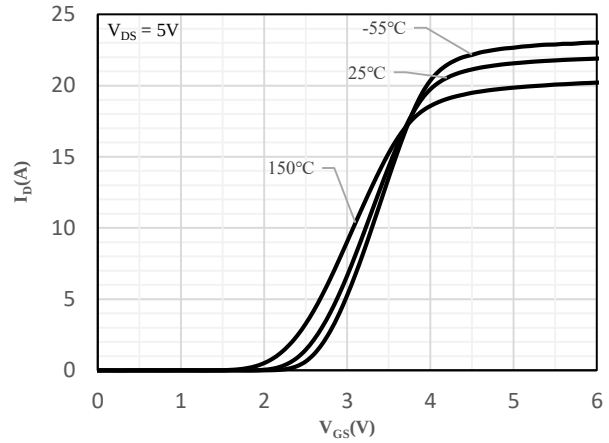
Fig 8 Transfer Characteristics
