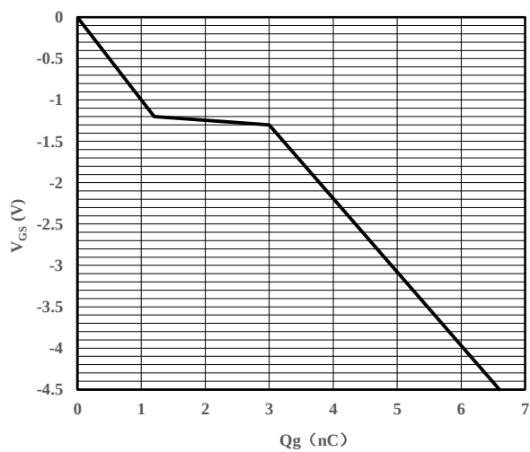
Fig 10 Gate-Charge Characteristics
