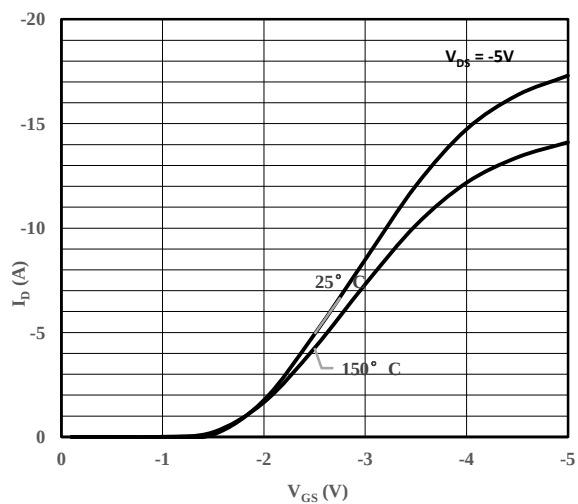
Fig 9 Transfer Characteristics
