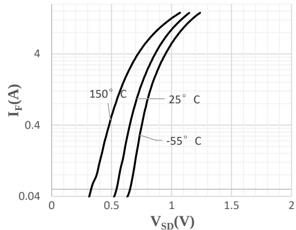
Fig 4 Body-Diode Characteristics
