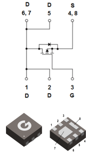
DFN2020-6L
