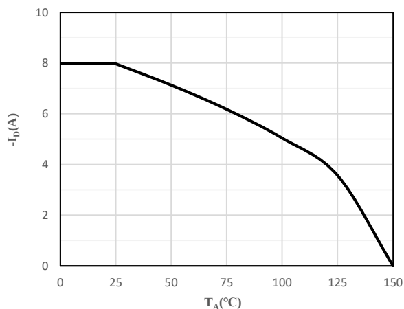
Fig 2 Drain Current
