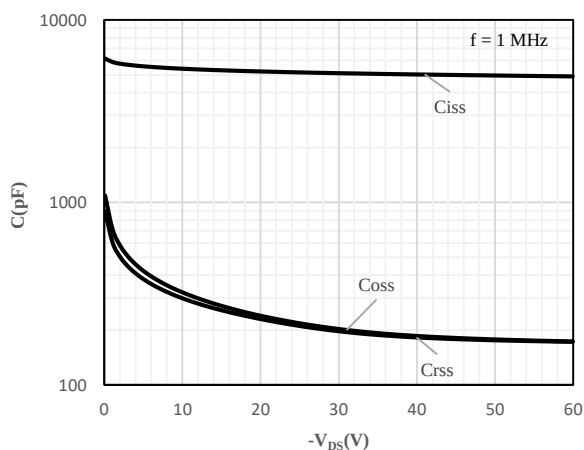
Fig 9 Capacitance Characteristics
