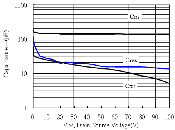
Fig 7 Capacitance Characteristics
