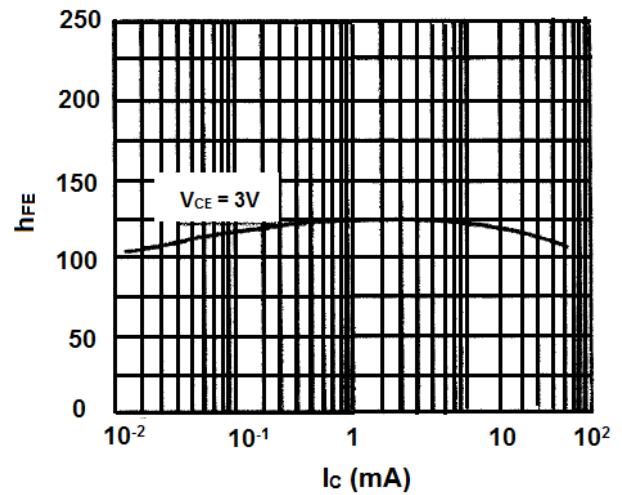
Fig. 4 DC Current vs. Collector Current
