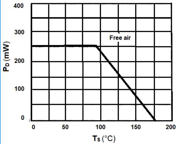
Fig. 1 Total Power Dissipation vs. Ambient Temperature
