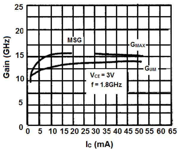
Fig. 6 Gain vs. Function of Collector Current
