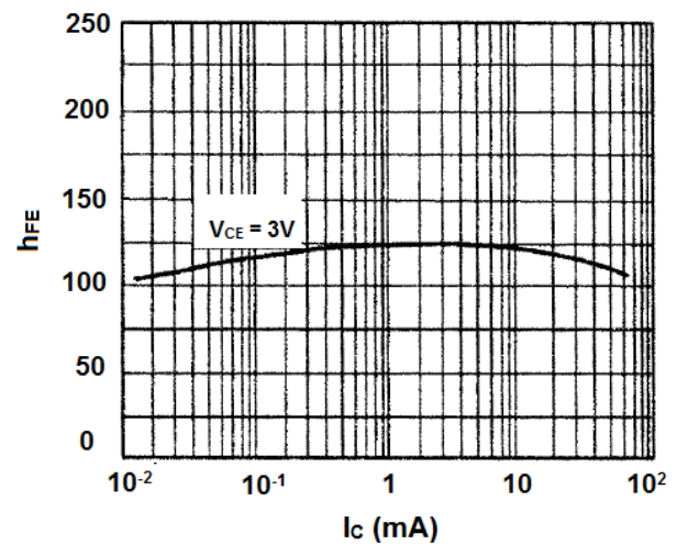
Fig. 4 DC Current vs. Collector Current
