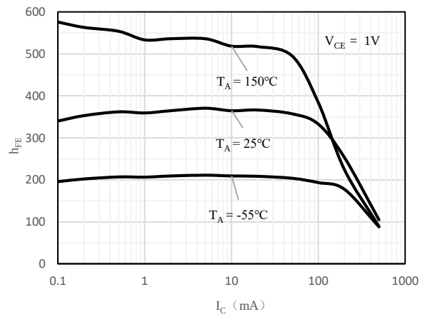
Fig 2 h_{FE} vs. I_C (BCW66G)
