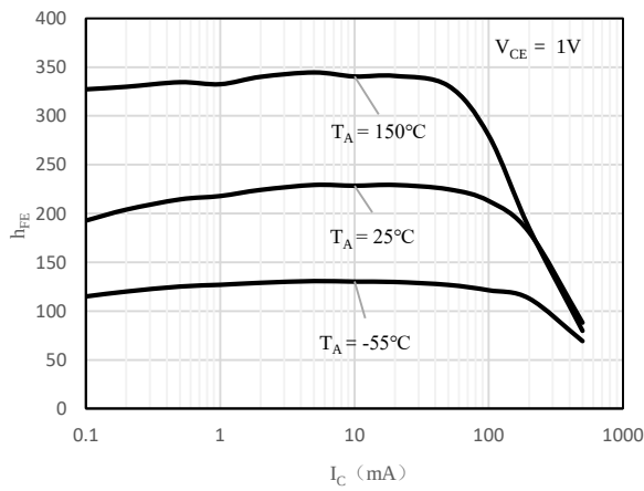
Fig 1 h_{FE} vs. I_C (BCW66F)
