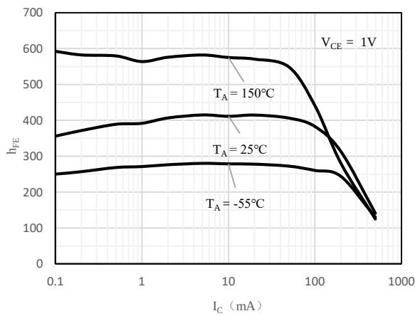
Fig 3 h_{FE} vs. I_C (BCW66H)
