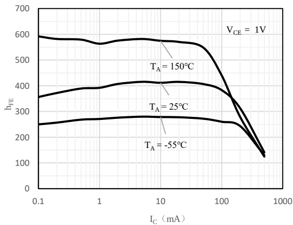
Fig 3 h_{FE} vs. I_C (BCW65C)
