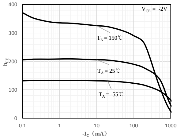
Fig 1 h_{FE} vs. I_C (BCP51/52/53-16)
