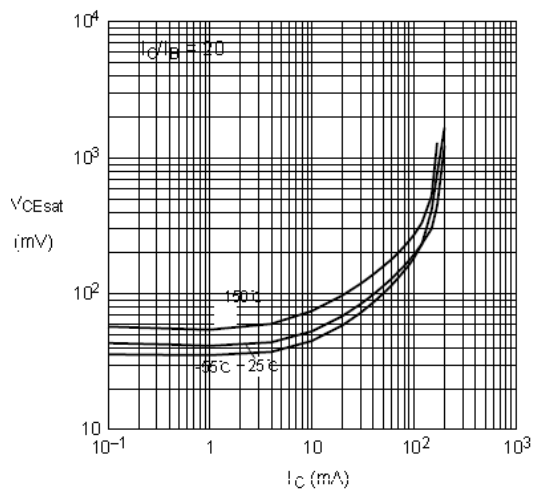
Fig 3 Collector-emitter saturation voltage as a function of collector current
