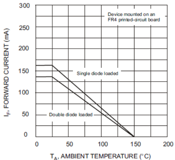
T_A , AMBIENT TEMPERATURE ( ^\circ\text{C} ) Fig. 2 Current Derating Curve
