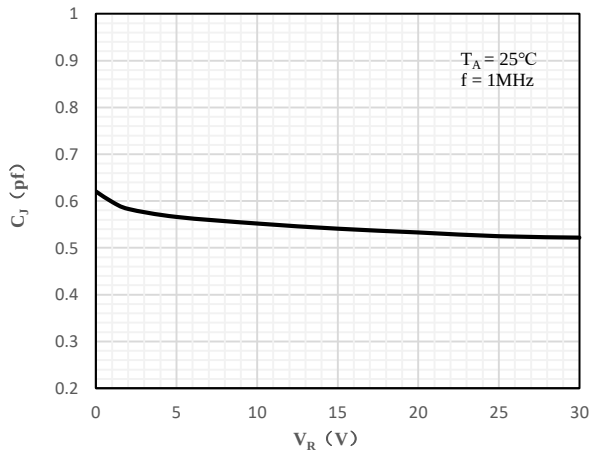
Fig 3 Typical Capacitance vs. Reverse Voltage
