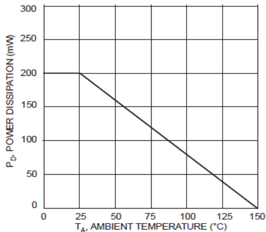
Fig. 1 Power Derating Curve, Total Package
