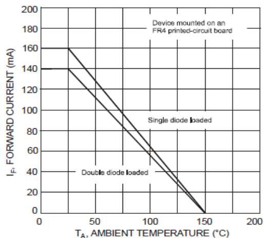
Fig. 4 Current Derating Curve, Per Element
