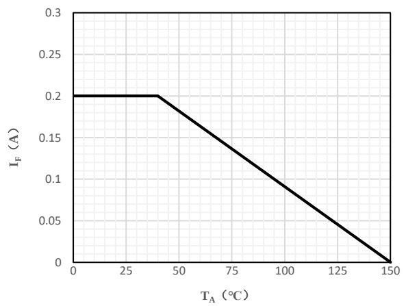
Fig 2 Derating Curve
