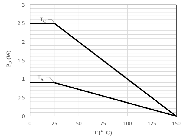
Fig 6 P_D vs. T
