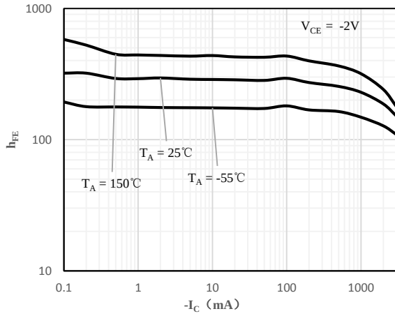
Fig 1 h_{FE} vs. I_C (Y: 160-320)
