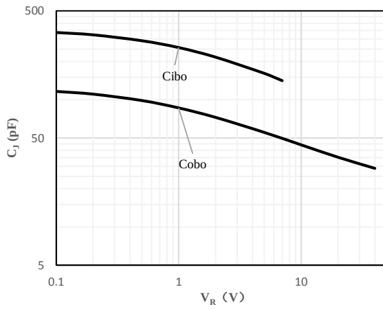
Fig 7 C_J vs. V_R
