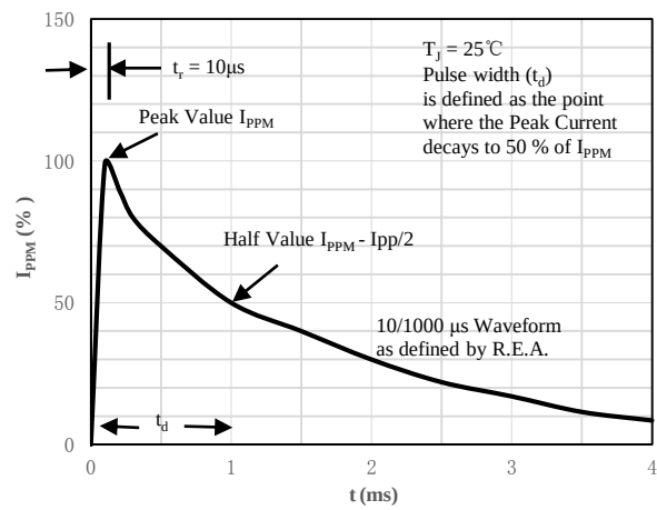
Fig 2 Pulse Waveform
