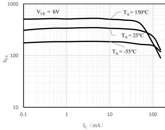
Fig 1 h_{FE} vs. I_C (R)
