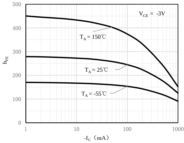
Fig 1 h_{FE} vs. I_C (R:160-320)
