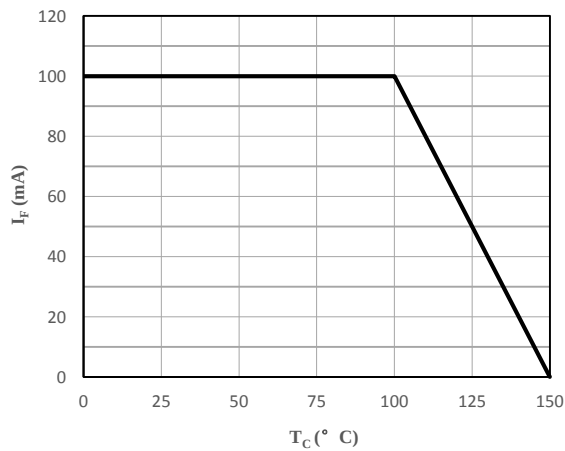
Fig 5 Current Derating
