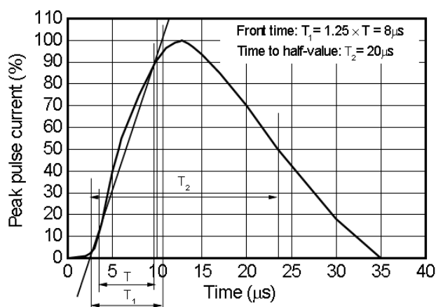
Fig3. 8/20 \mu\text{s} waveform per IEC61000-4-5
