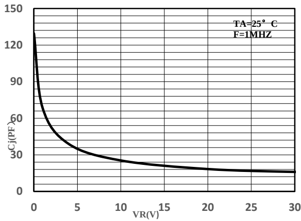
Fig.3-Capacitance Characteristics
